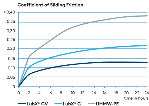
Coefficient of sliding friction under dry conditions, validated on Roechling application-level tribology test apparatus, speed: 0.5 m/s, surface pressure 0.5 MPa, test time 24 hours
