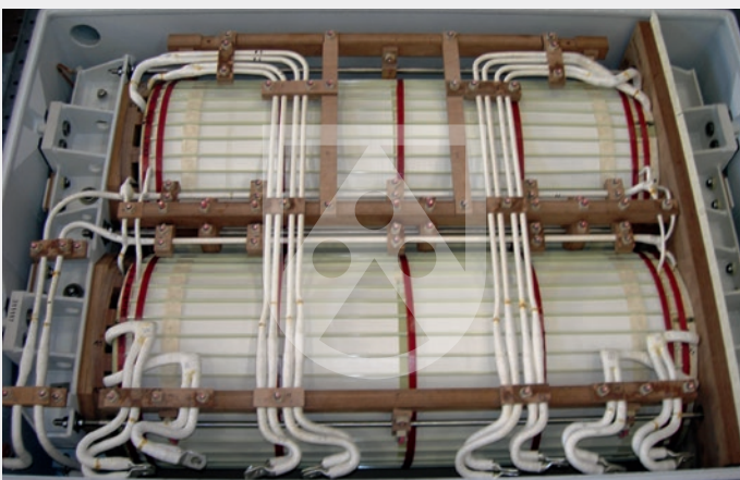
Traction transformer
