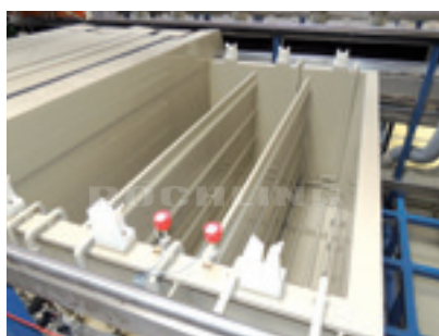
Polystone® P homopolymer grey Process tanks in a plastic electroplating
